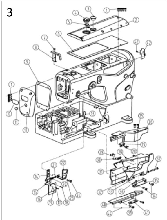
三、罩壳部件(Cover assemblies)
